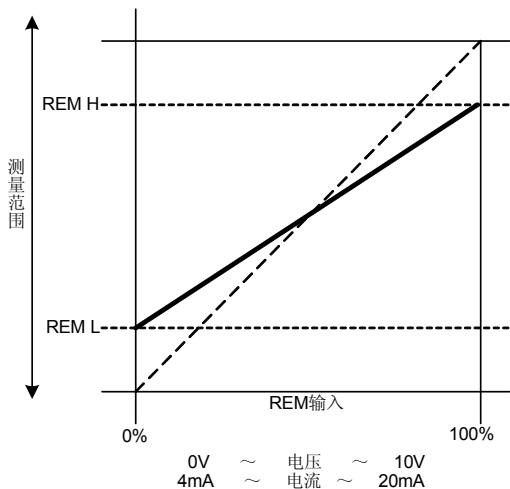
(1) RM_L < RM_H
